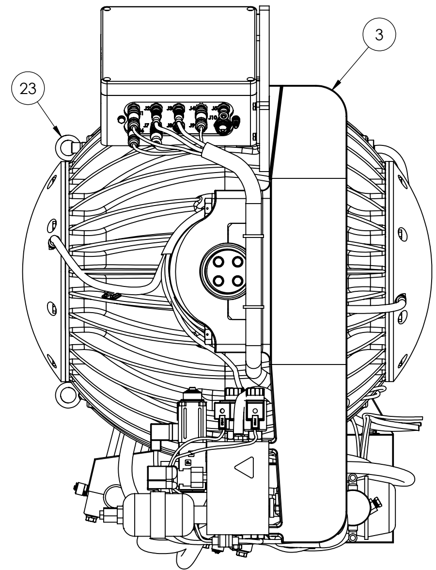
STARBOARD SIDE VIEW
