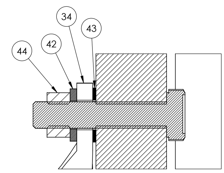
SECTION D-D GROUND STUDS DETAIL
