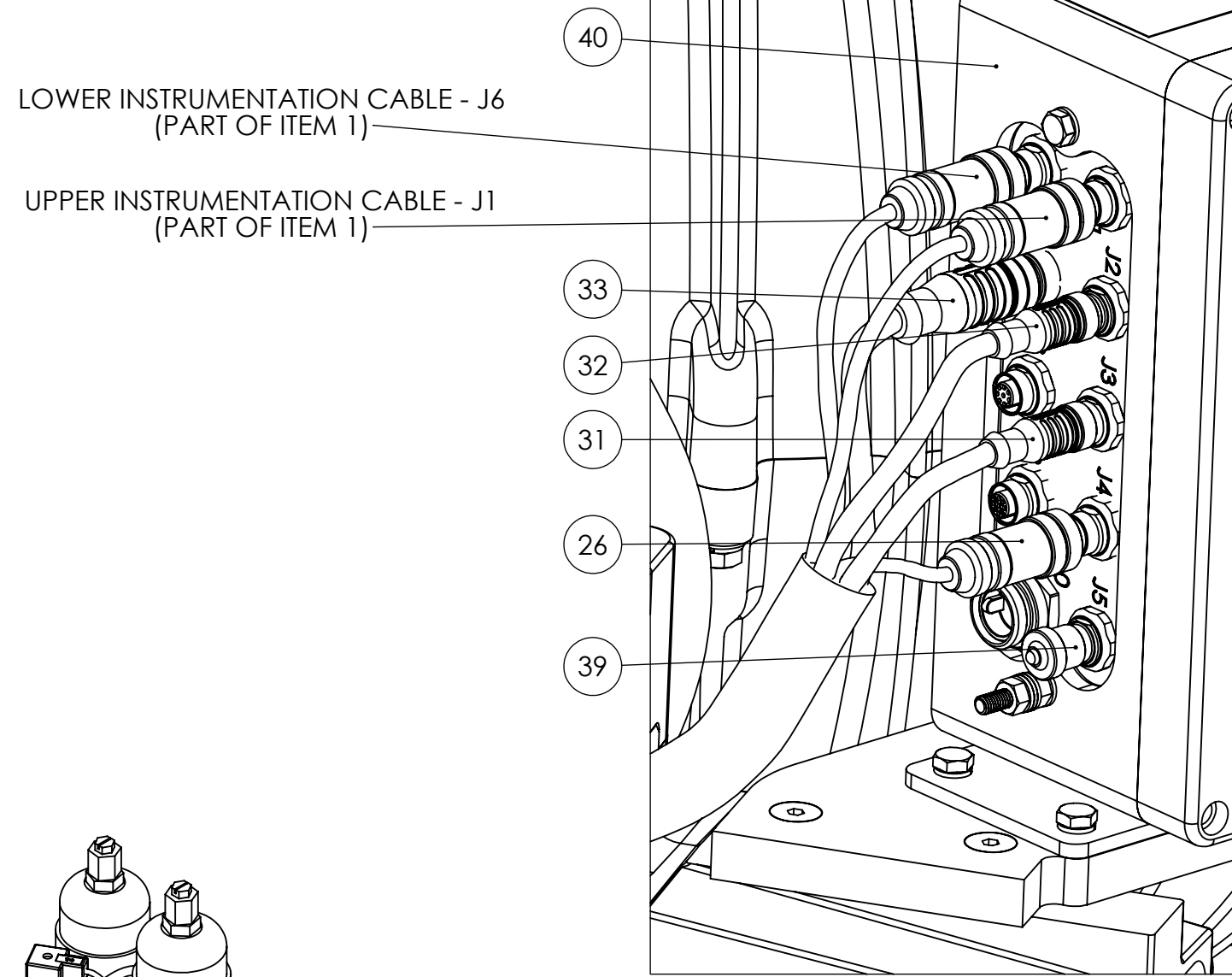
CABLE CONNECTIONS TO CONTROL BOX
