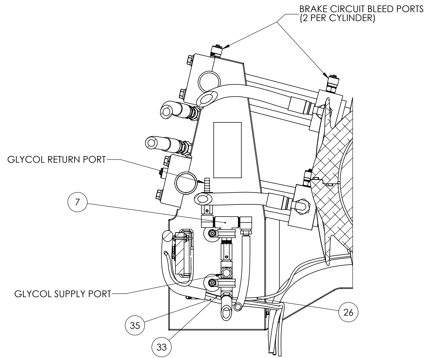
SECTION B-B VIEW OF INBOARD FACE OF BRAKE SADDLE ENCLOSURE-GIMBAL SHAFT SUB-ASSEMBLY NOT SHOWN
