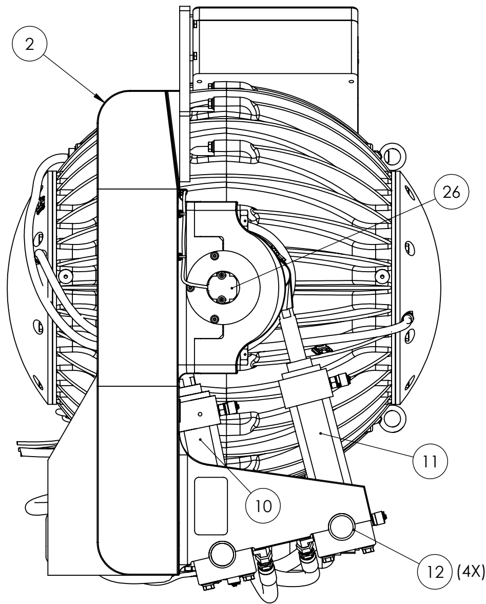
PORT SIDE VIEW
