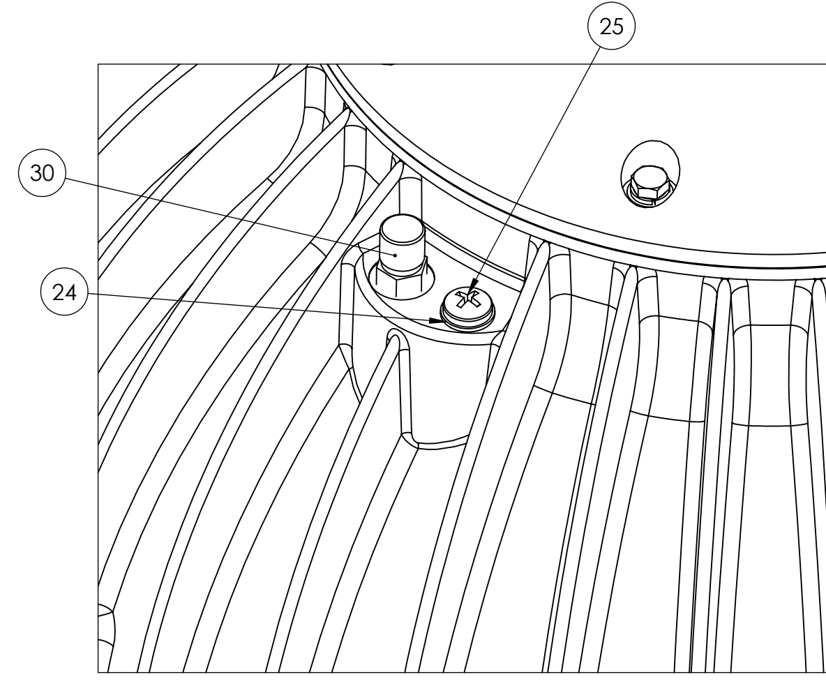
LIFTING POINT HARDWARE (2 PLACES) (ITEMS 24 & 25 SHIP LOOSE WITH GYRO ASSEMBLY)
