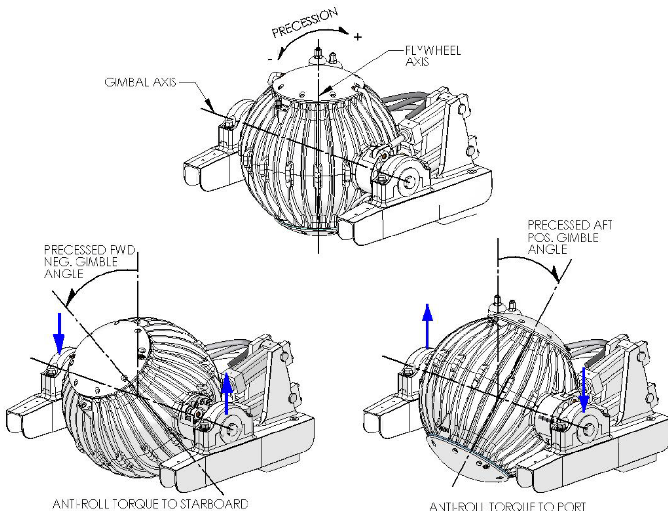
FIGURE 2 – GYRO PRECESSION
