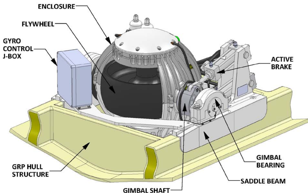
FIGURE 3 – GYRO ASSEMBLY
