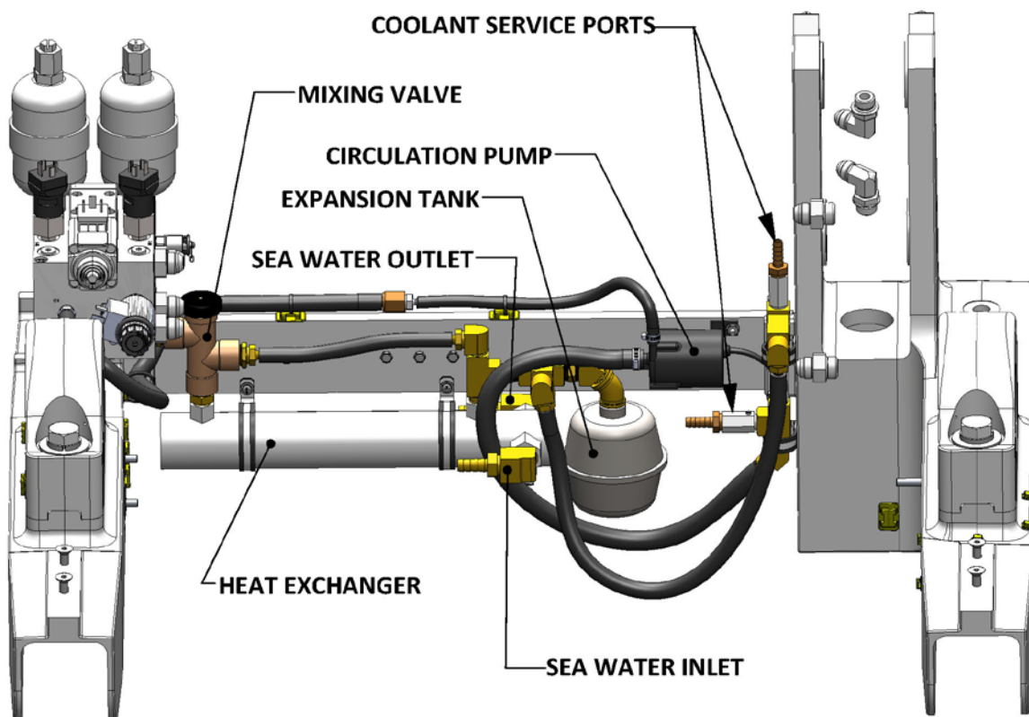
FIGURE 6 – COOLING SYSTEM COMPONENTS
