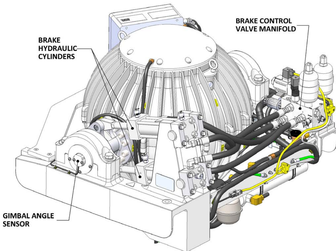
FIGURE 5 – BRAKE
