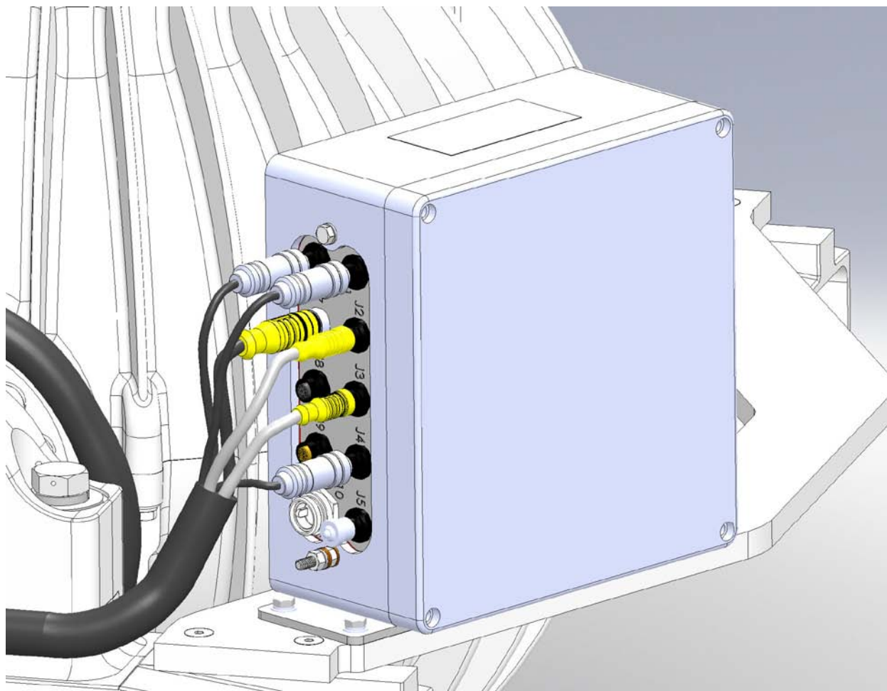
FIGURE 4 – GYRO MOUNTED CONTROL BOX
