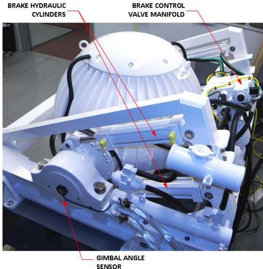
FIGURE 9 – BRAKE
