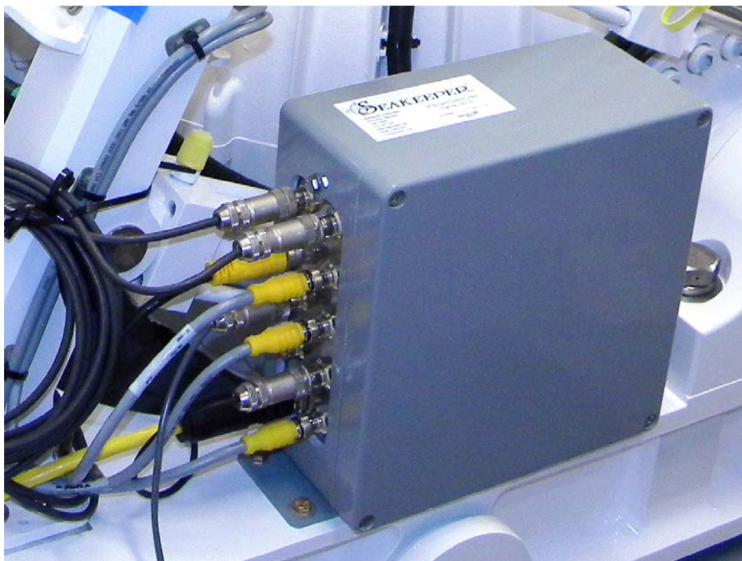
FIGURE 8 – GYRO MOUNTED CONTROL BOX
