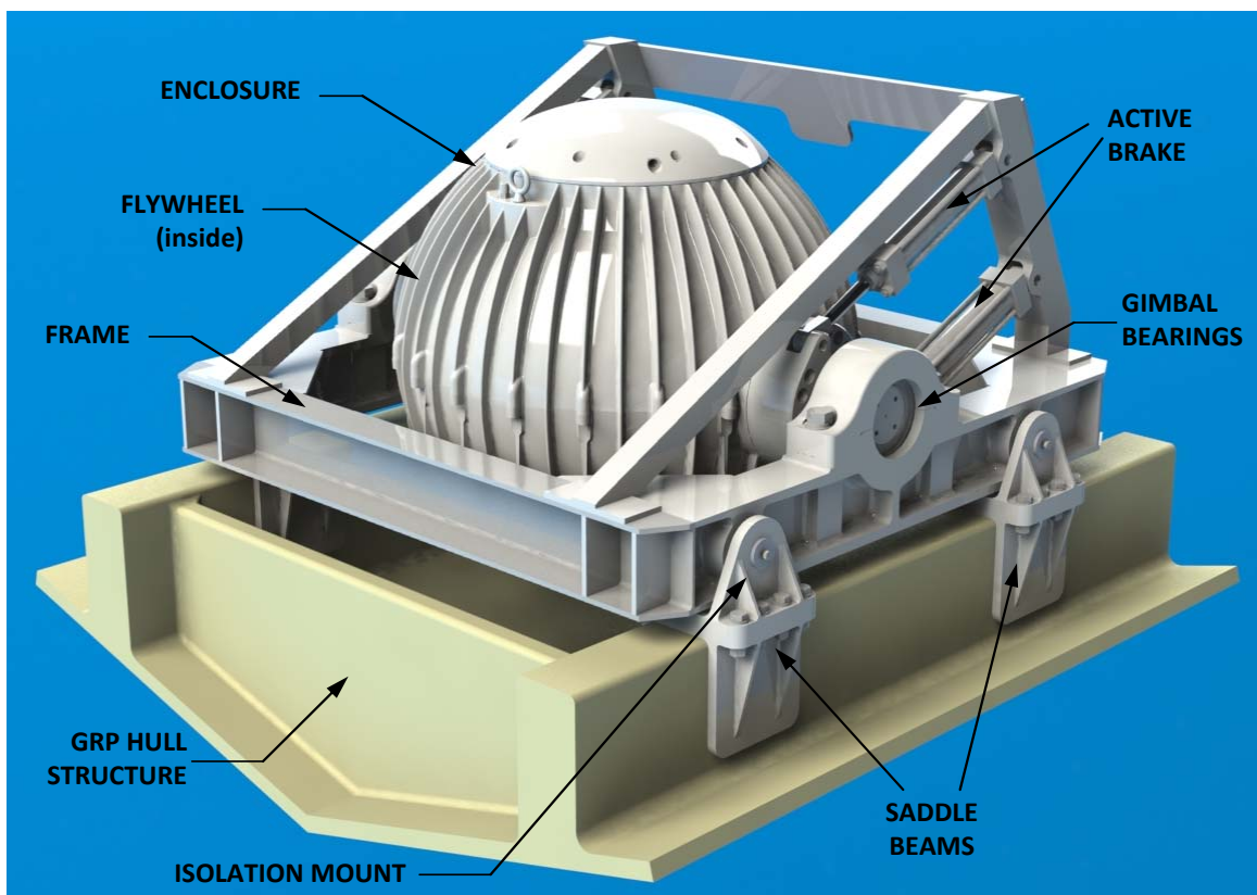
FIGURE 3 – GYRO ASSEMBLY
