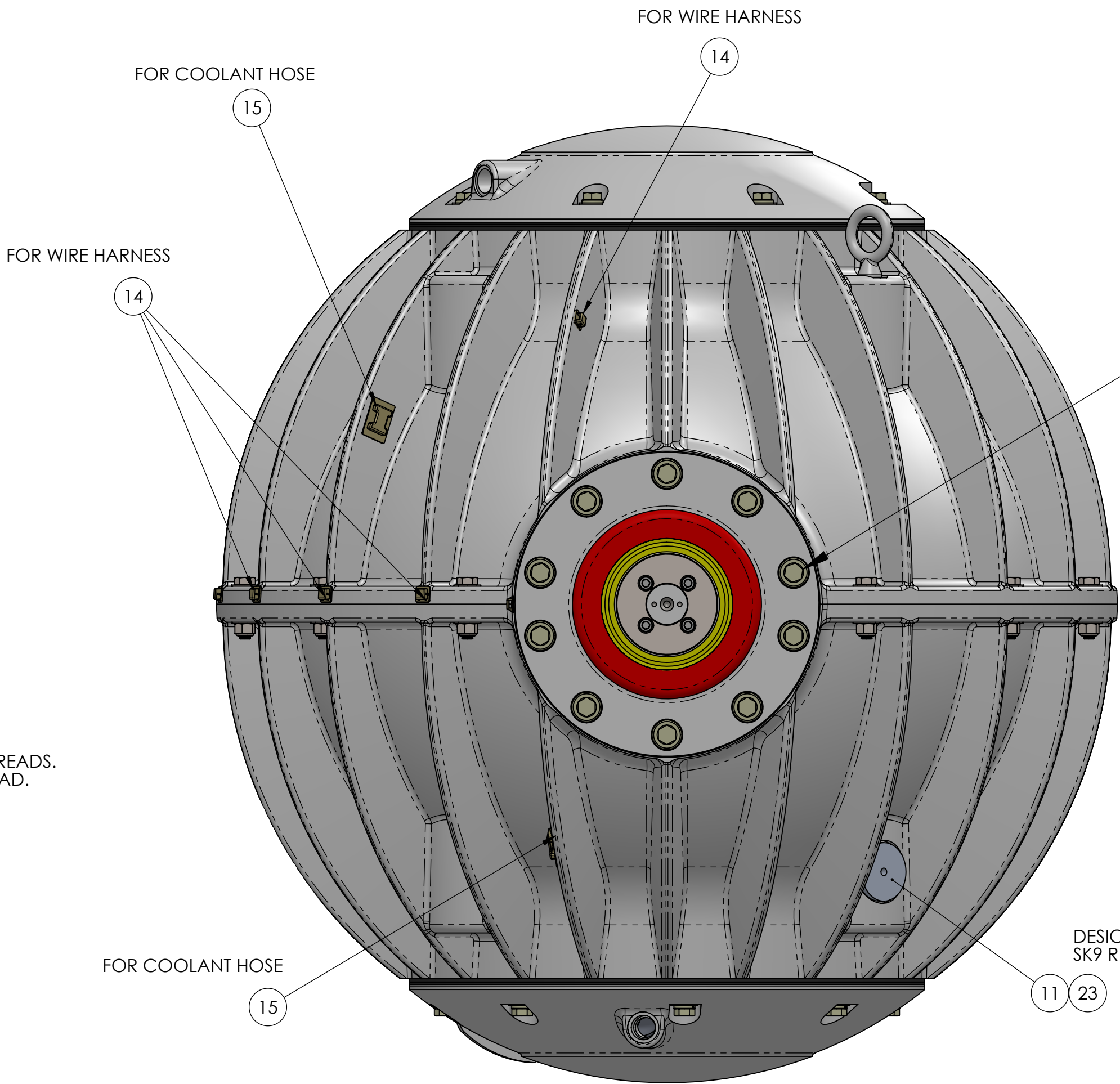
NON- BRAKE SIDE CLICK BOND LOCATIONS
