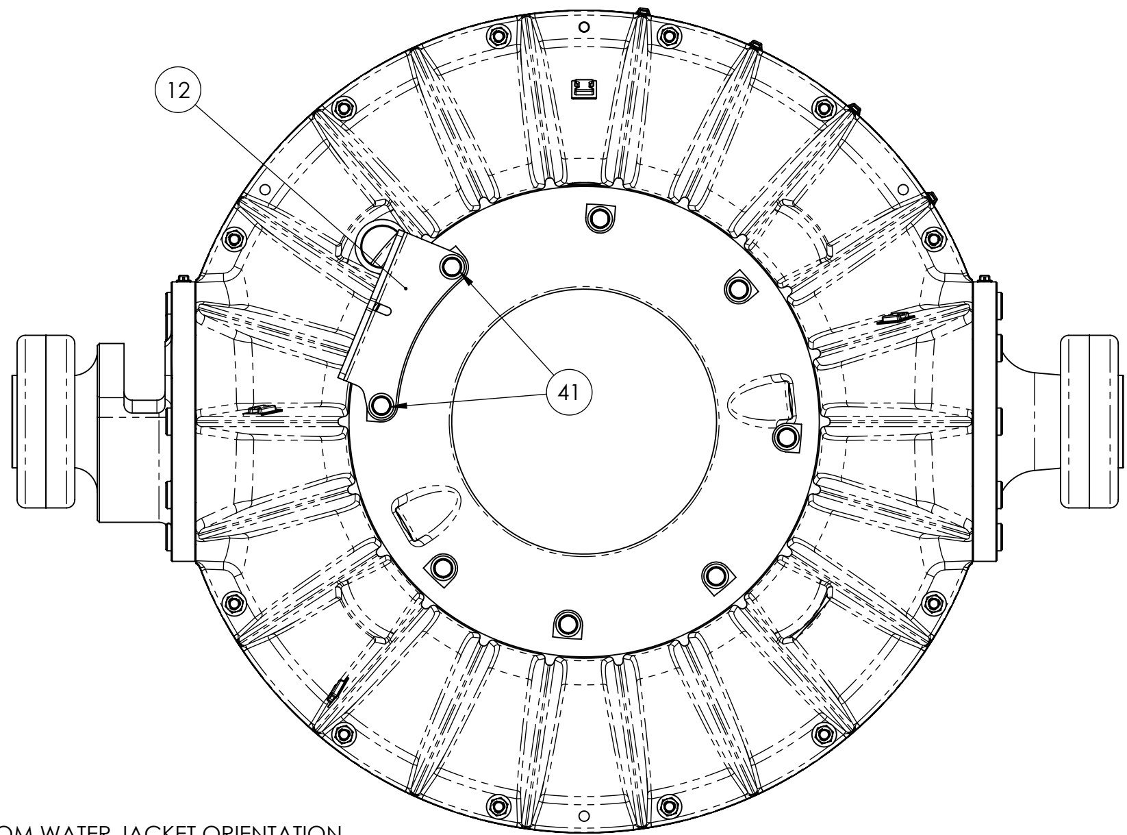
BOTTOM WATER JACKET ORIENTATION
