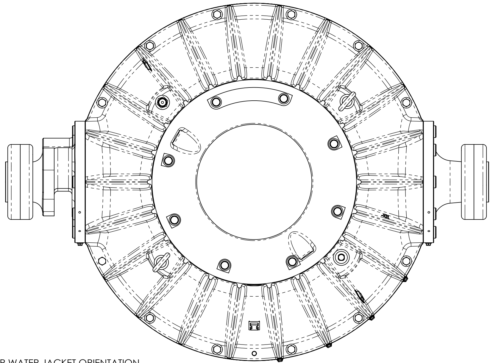
TOP WATER JACKET ORIENTATION
