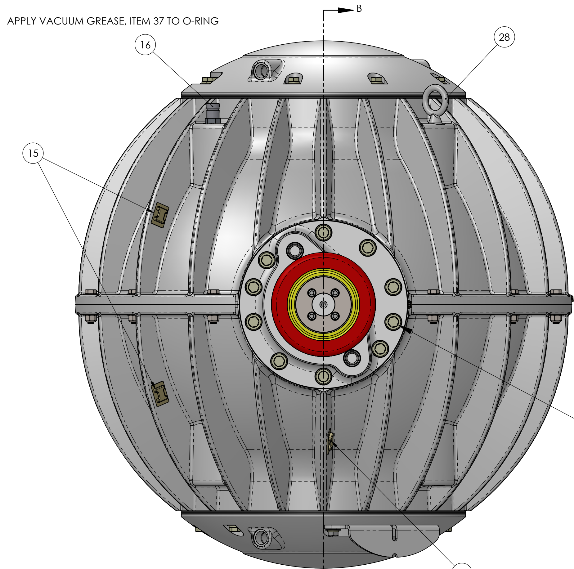
BRAKE SIDE CLICK BOND LOCATIONS
