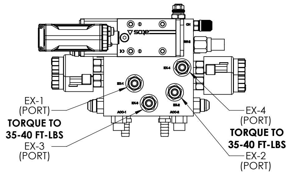
FACE VIEW
