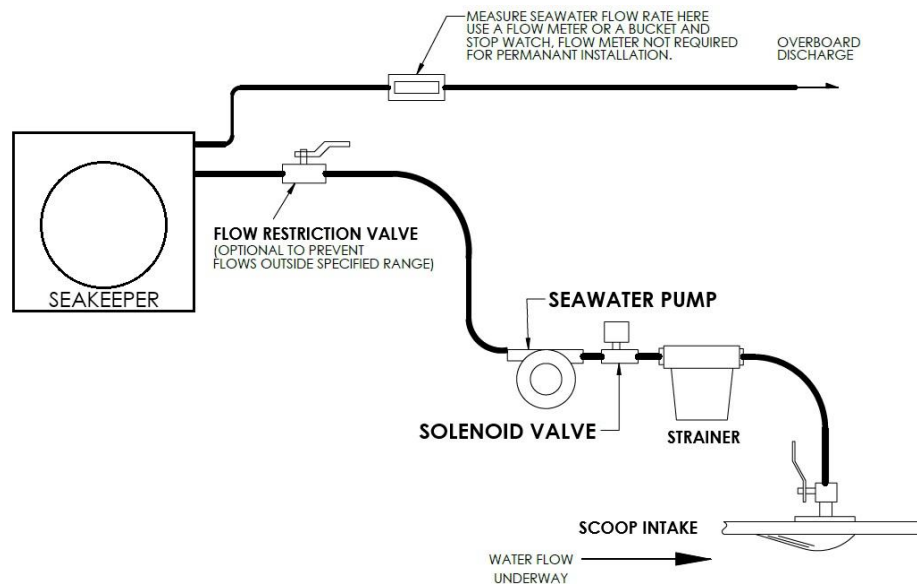
Figure 3: Simplified schematic of an ideal seawater plumbing arrangement
