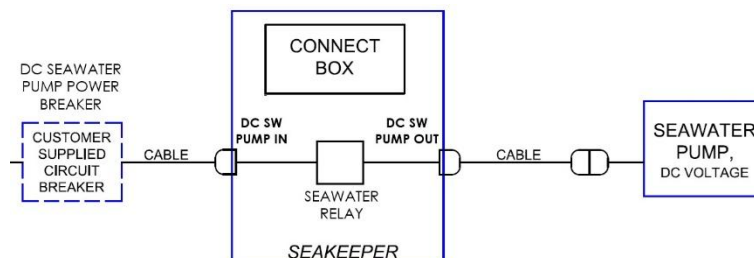
Figure 2: DC Seawater Pump power schematic
