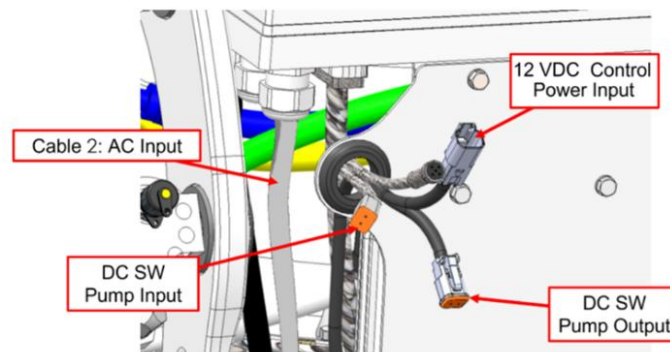
Figure 1: Power cables, including DC seawater pump power cables
