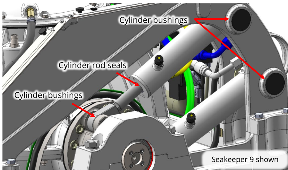
Figure 9: brake cylinder details shown.
