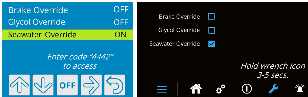
Figure 6: Hidden override screen shown.
