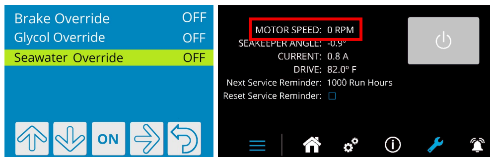
Figure 1: Service screen shown with motor speed highlighted
